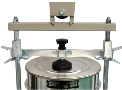
Detail of the fast clamping system
